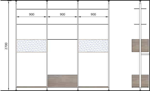
Kit Libreria Bookshelves Kit MN/CMSL.003
