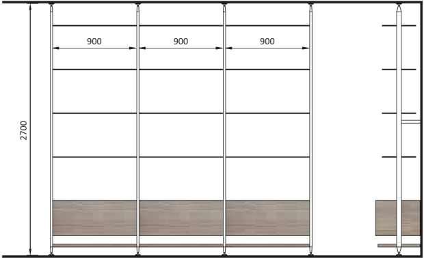
Kit Libreria Bookshelves Kit MN/CMSL.001xx
