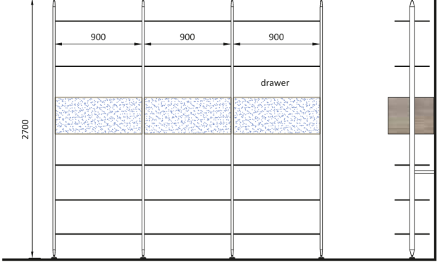
Kit Libreria Bookshelves Kit MN/CMSL.002xx
