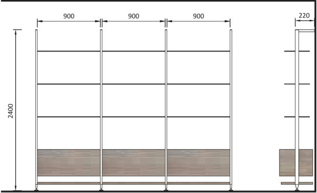
Kit Libreria Bookshelves Kit MN/CMPL.001xx
