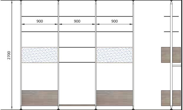
Kit Libreria Bookshelves Kit MN/CMSL.004
