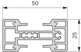
Profilo verticale strutturale chiuso Closed vertical structural profile
