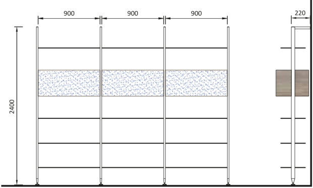
Kit Libreria Bookshelves Kit MN/CMPL.002xx
