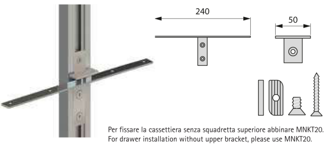
Kit cassetiera Kit drawer
