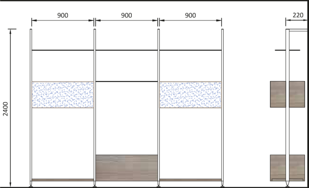
Kit Libreria Bookshelves Kit MN/CMPL.003
