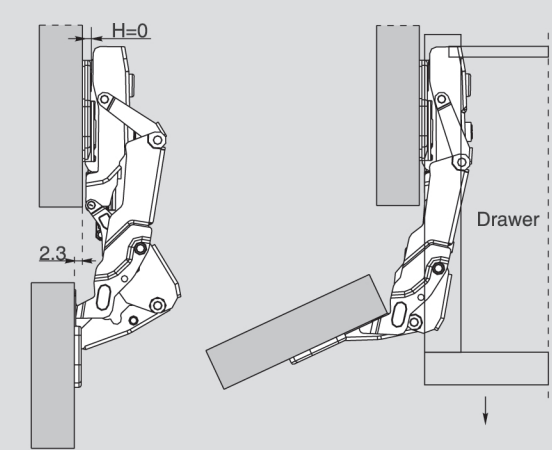
Full overlay C=0
