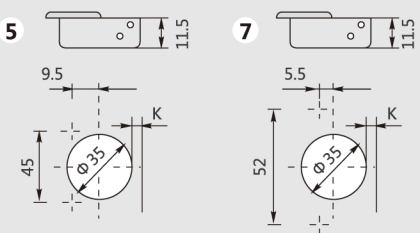
C80 Series snap-on cam-adjustable soft-close 30° angled hinges
