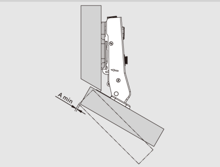
Space needed to open the door
