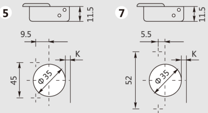
Φ 35mm Hinge cup types
