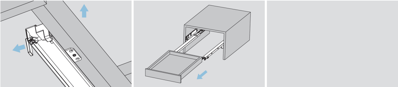
For removal, pull out the locking pin from the drawer side. Lift the drawer and pull it out from the cabinet.
