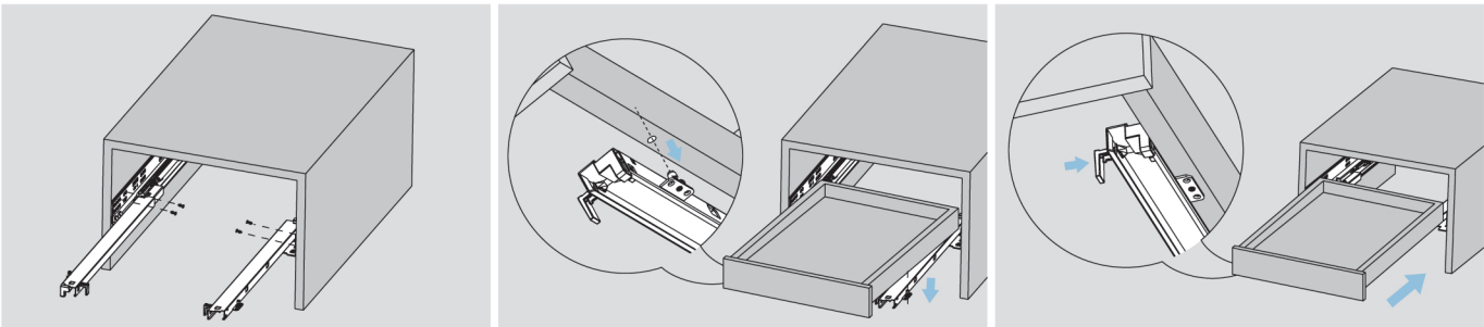
Fix the slide onto the cabinet. Pull out the drawer member of the slide from the cabinet, lay the drawer onto the slide. Press the locking pin into the drawer side to lock the position of the drawer.
