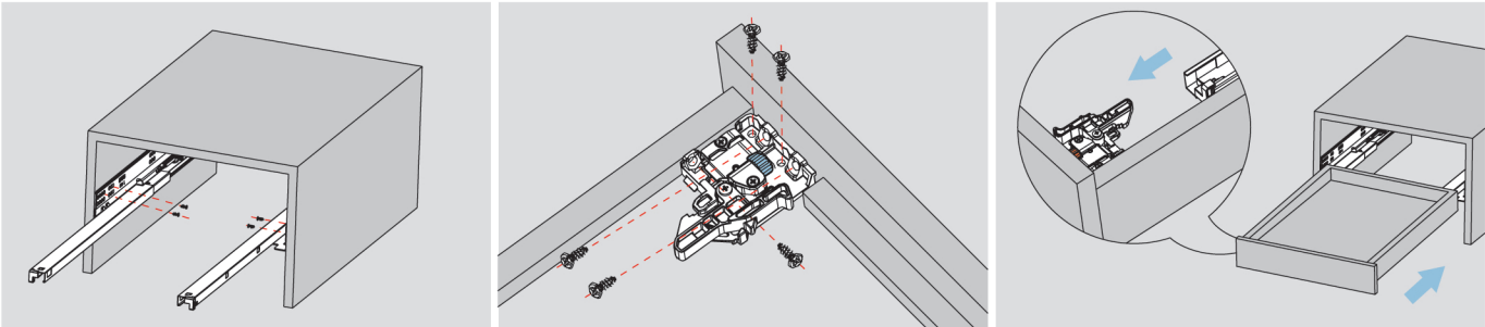
Fix the slide onto the cabinet. Fix the locking device onto the drawer bottom. Lay the drawer bottom onto the slide then push the drawer into the cabinet.
