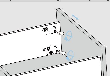
Left&right adjustment
