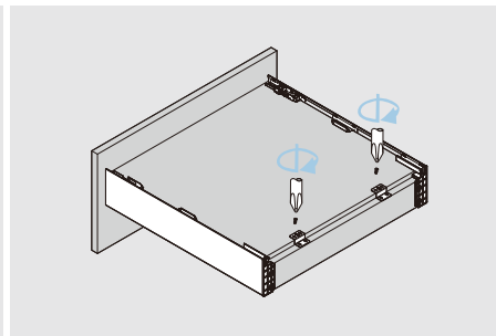
Fixing-brackets assembly
