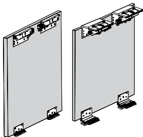
Install top and bottom rollers onto outer and inner doors
