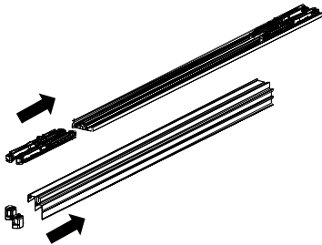
Insert the damper into top track Insert the bottom stopper into bottom track
