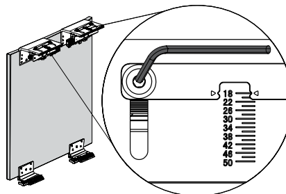
Choose your door thickness
