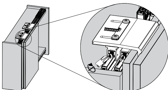
Level the outer and inner doors
