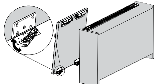
Disengage the locking device on bottom roller before mounting the inner door
