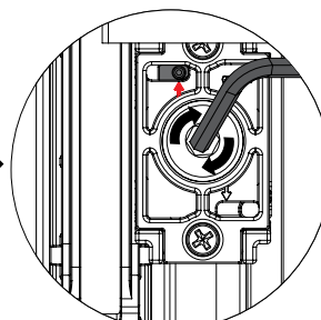
Turn the screw clockwise with a 3mm allen key to engage the locking devices on the top rollers of the outer and inner doors
