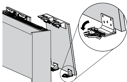
Disengage the locking device on bottom roller before mounting the outer door
