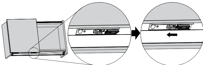
Engage the locking device on bottom roller after mounting the inner door on wardrobe
