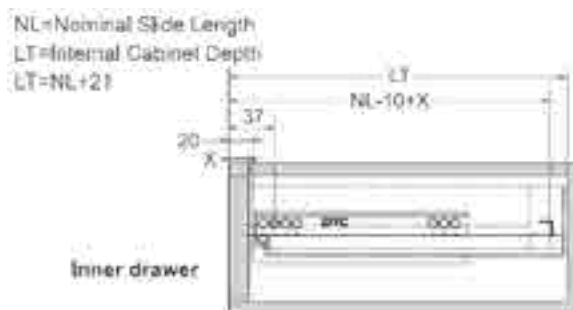
Installation Dimensions(mm)
