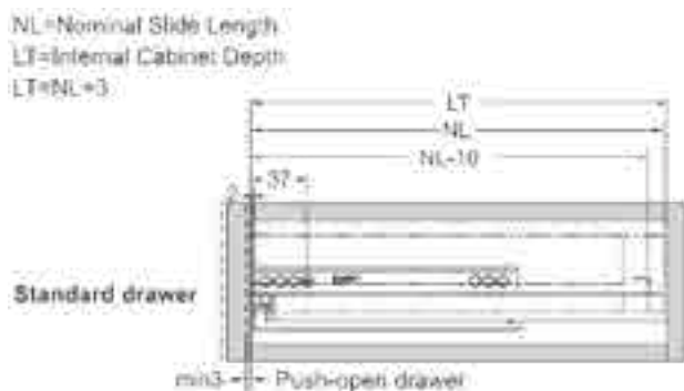
Installation Dimensions(mm)
