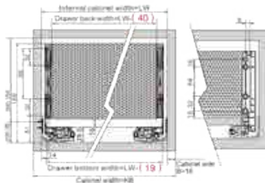
Installation Dimensions(mm)
