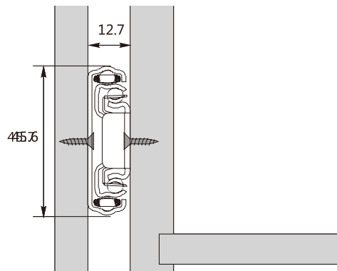
Installation Dimensions(mm)
