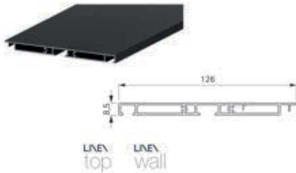
Front line profile
