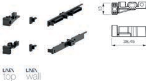
Free shelf connection kit
