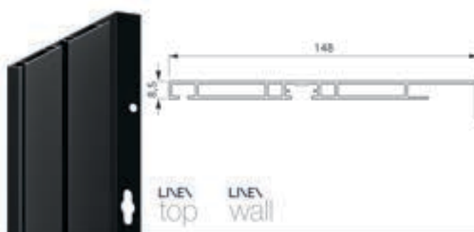
Free shelf profile
