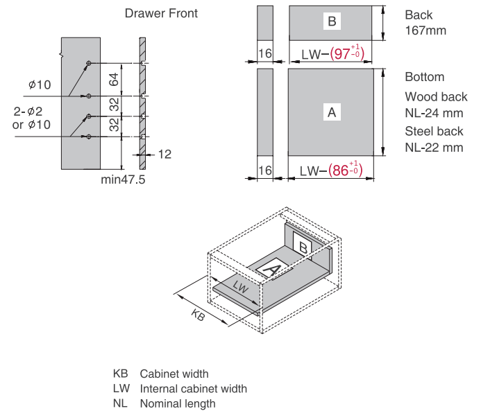
Drawer Front, Back and Bottom Dimensions(mm)
