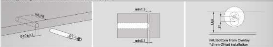
Insert-type Magnetic Push Latch Installation Dimensions(mm)
