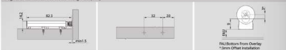
Magnetic Push Latch with In-line Fixing Plate(mm)
