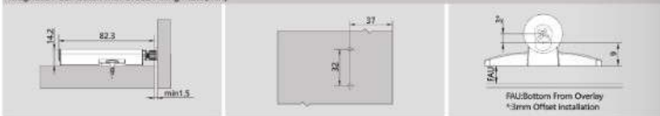
Magnetic Push Latch with Cross Fixing Plate(mm)
