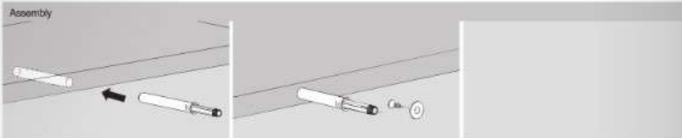
Magnetic Push Latch with In-line Fixing Plate(mm)
